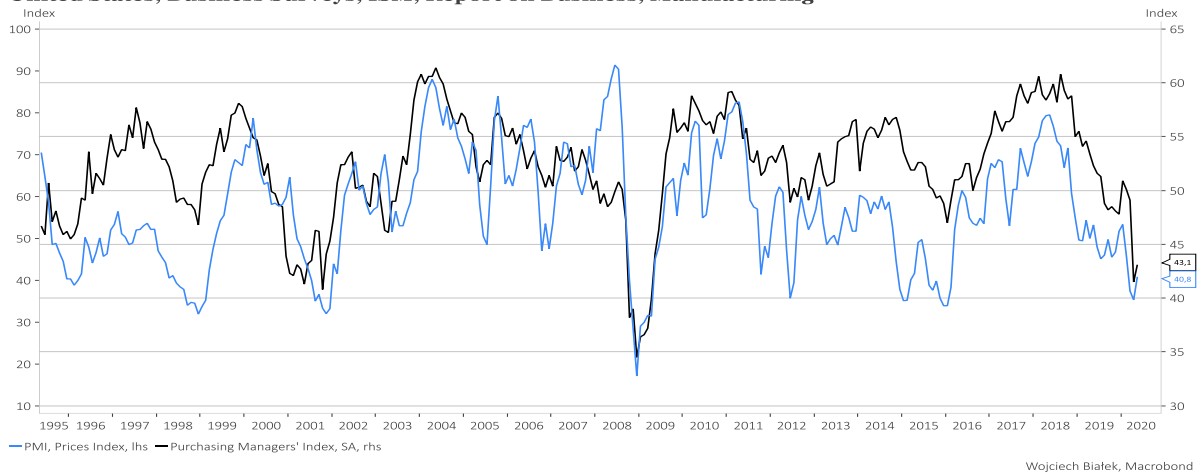
United States, Business Surveys, ISM, Report on Business, Manufacturing
