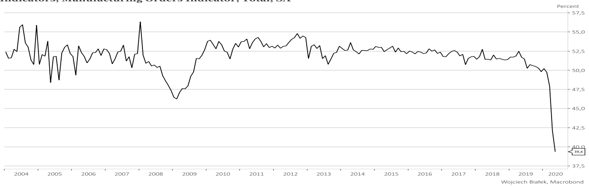
Mexico, Business Surveys, INEGI National Institute of Geography & Statistics, Manufacturing View Indicators, Manufacturing Orders Indicator, Total, SA
